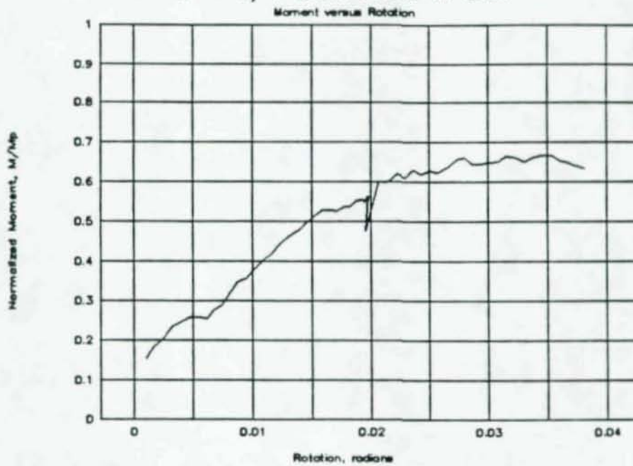
Figure A-6: Normalized moment versus rotation for 5-bolt specimen
