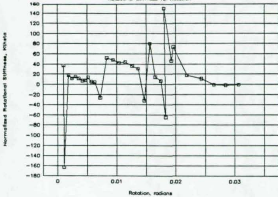
Figure 4-8: Rotational stiffness behavior of 9-bolt specimen
