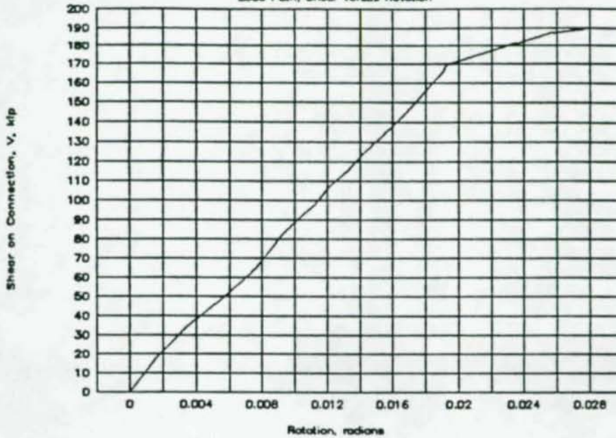
Figure A-3: Load path for 7-bolt specimen
