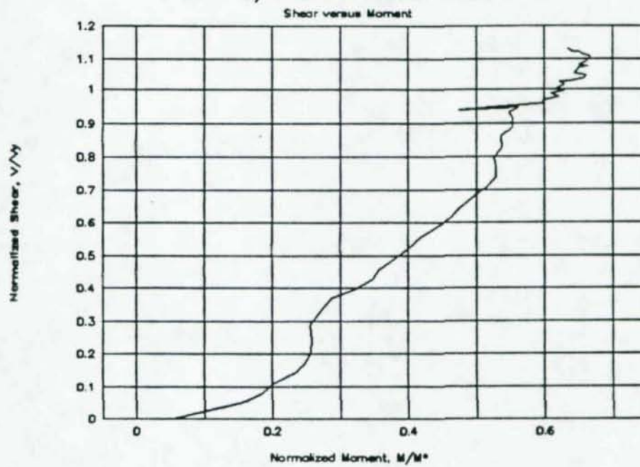
Figure A-10: Normalized shear-moment behavior for 5-bolt specimen
