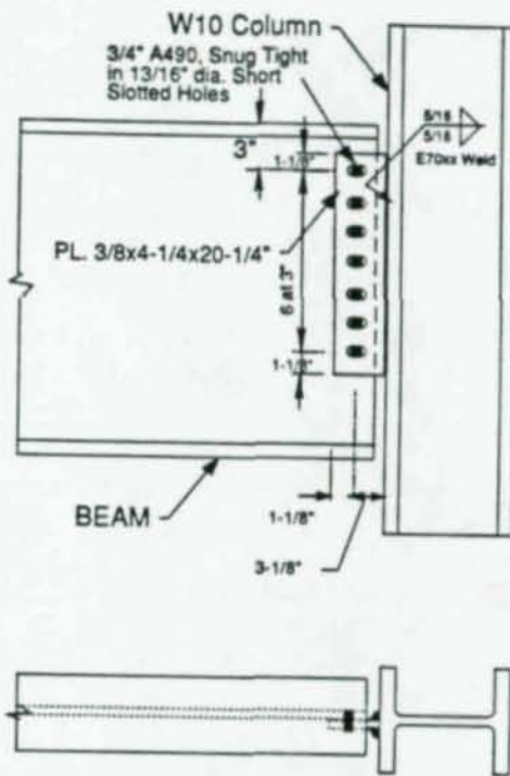
Figure 2-3: Seven-bolt test specimen
