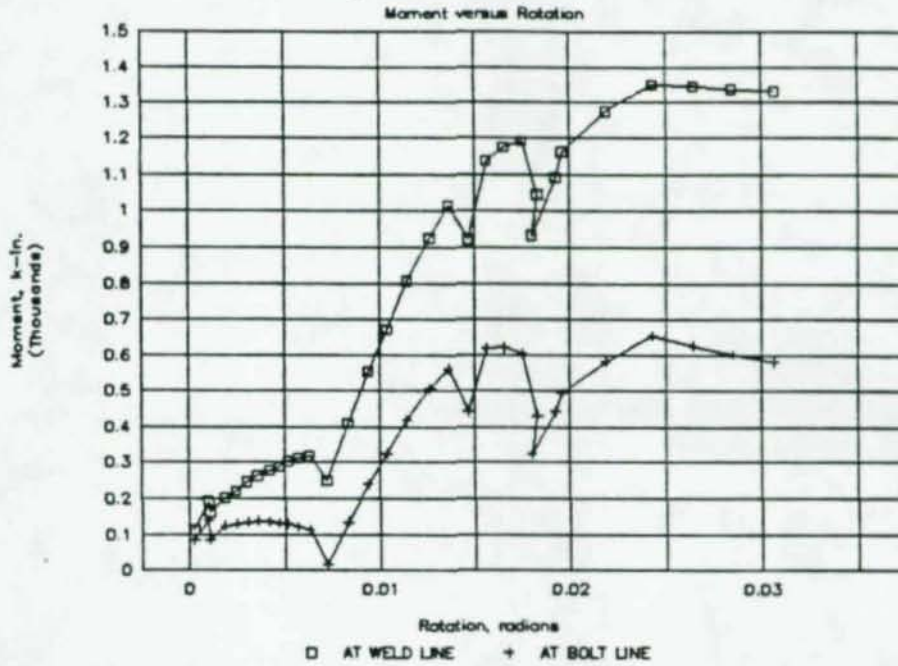
Figure 4-4: Moment-rotation behavior of 9-bolt specimen
