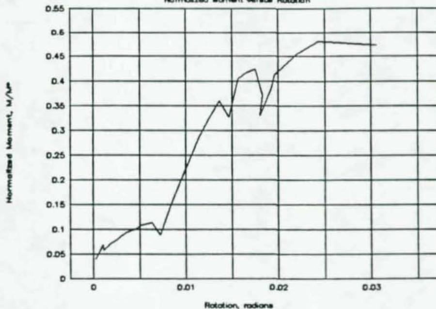
Figure A-8: Normalized moment versus rotation for 9-bolt specimen
