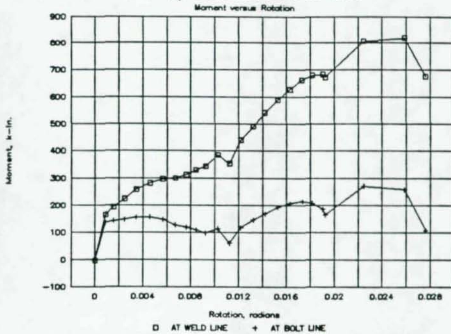
Figure 4-3: Moment-rotation behavior of 7-bolt specimen
