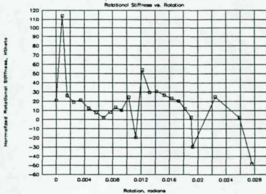
Figure 4-7: Rotational stiffness behavior of 7-bolt specimen
