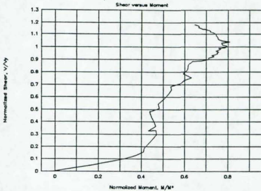
Figure A-9: Normalized shear-moment behavior for 3-bolt specimen
