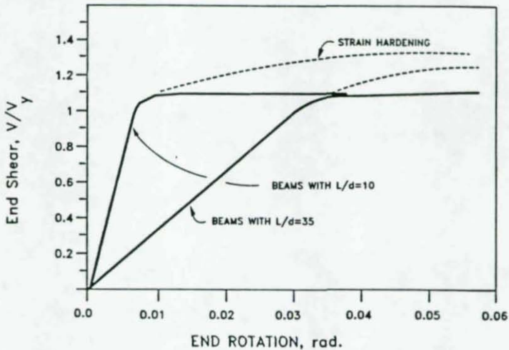
Figure 2-5: Shear-rotation curves of typical beams
