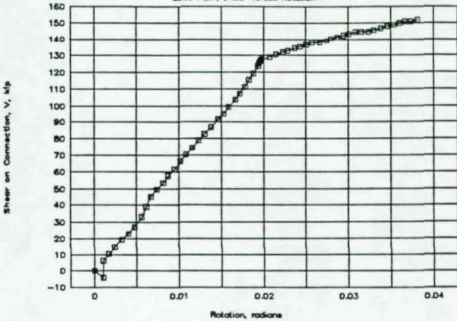
Figure A-2: Load path for 5-bolt specimen
