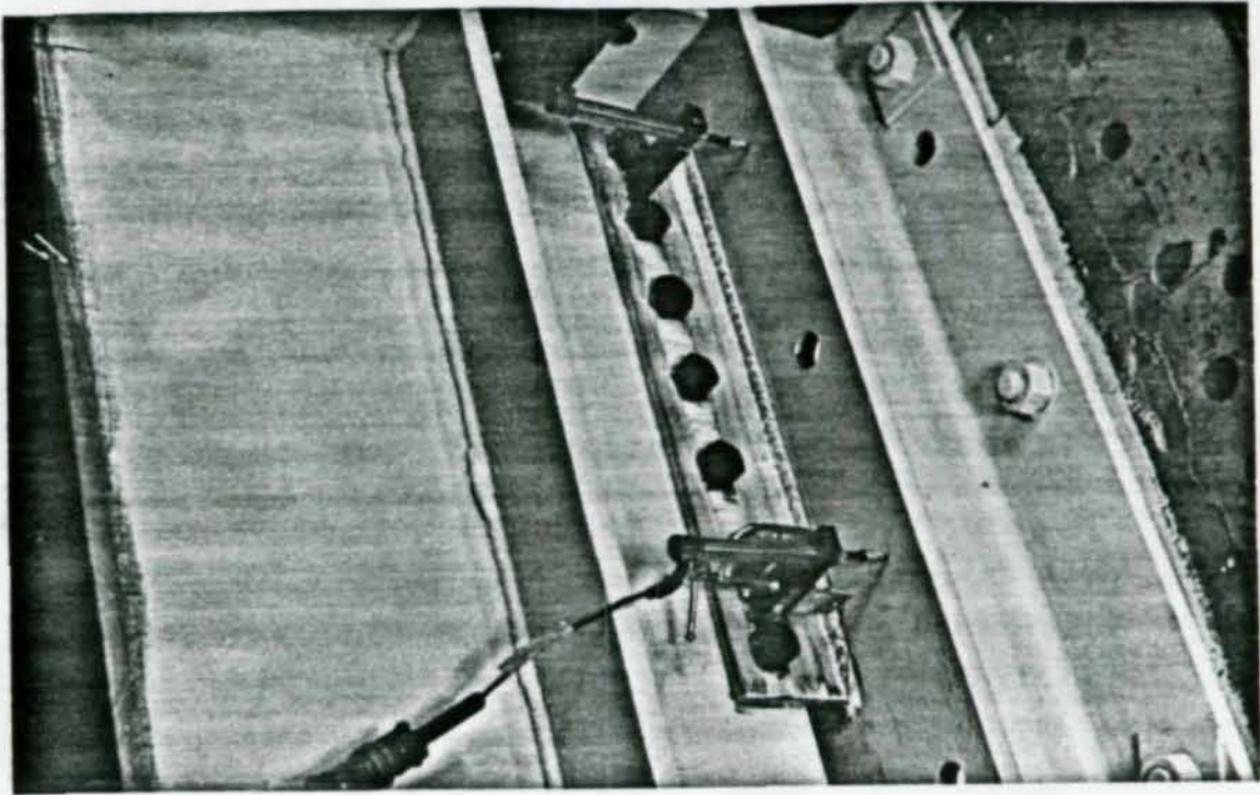
Figure 3-3: A view of seven-bolt specimen
