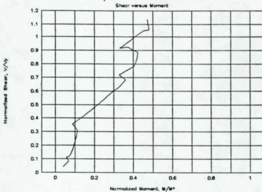
Figure A-12: Normalized shear-moment behavior for 9-bolt specimen
