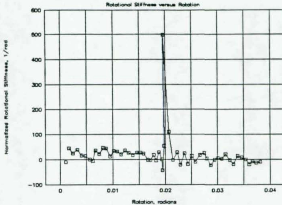
Figure 4-6: Rotational stiffness behavior of 5-bolt specimen
