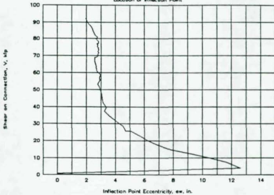
Figure 4-9: Reaction eccentricity behavior of 3-bolt specimen
