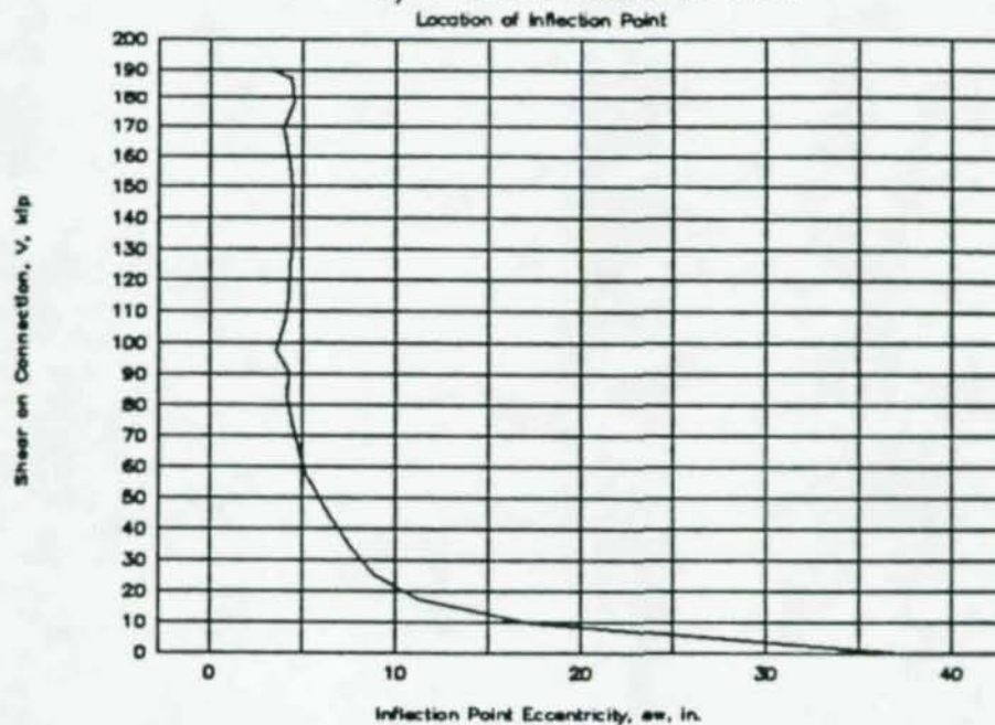
Figure 4-11: Reaction eccentricity behavior of 7-bolt specimen
