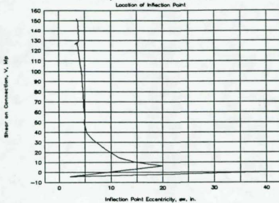
Figure 4-10: Reaction eccentricity behavior of 5-bolt specimen
