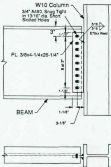
Figure 2-4: Nine-bolt test specimen
