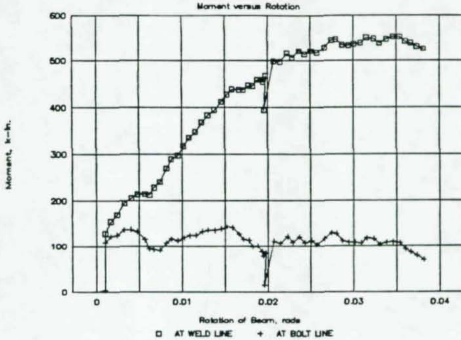
Figure 4-2: Moment-rotation behavior of 5-bolt specimen
