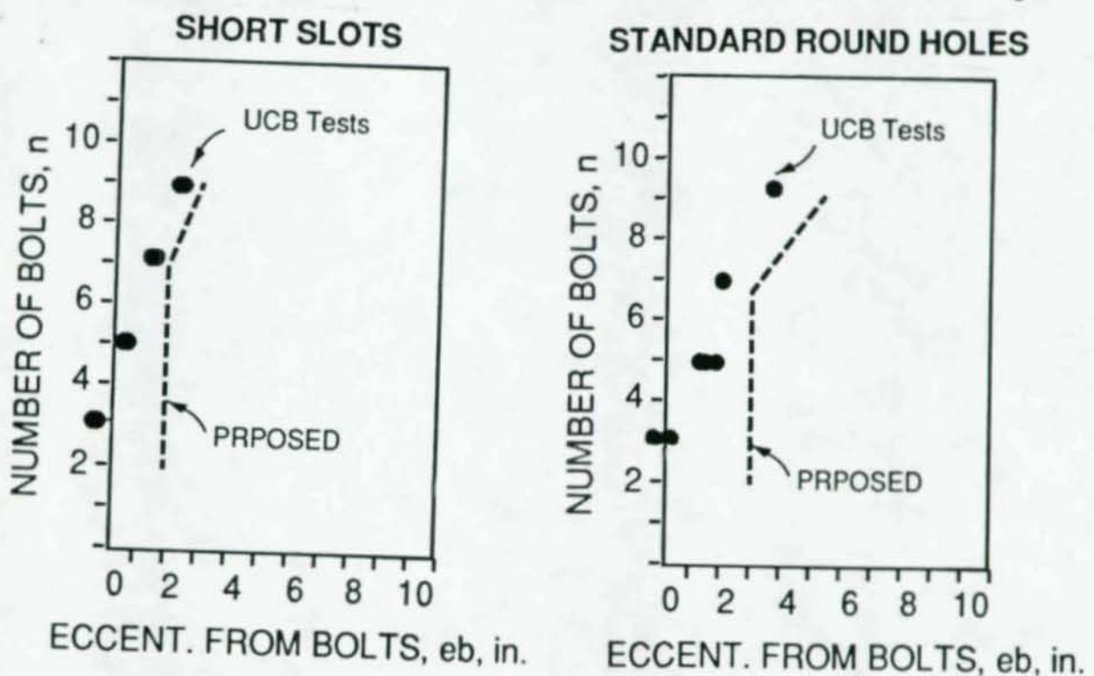
Figure 4-13: Eccentricity of point of inflection
