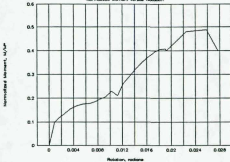
Figure A-7: Normalized moment versus rotation for 7-bolt specimen
