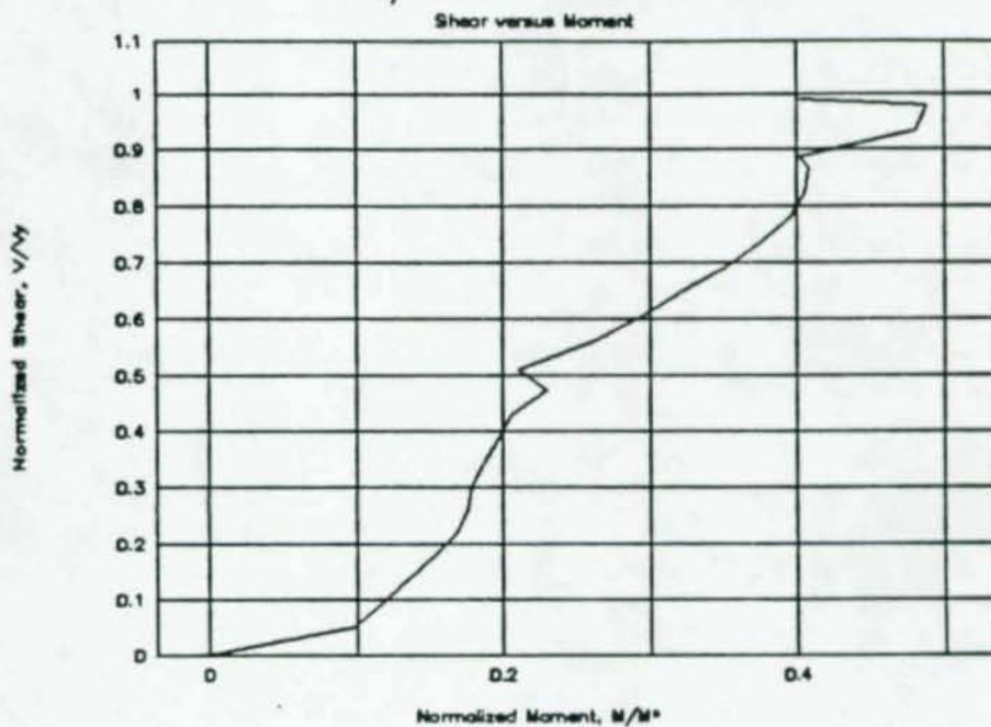
Figure A-11: Normalized shear-moment behavior for 7-bolt specimen
