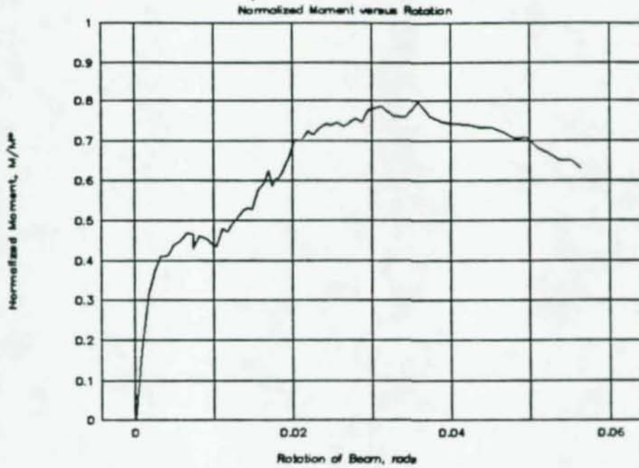
Figure A-5: Normalized moment versus rotation for 3-bolt specimen
